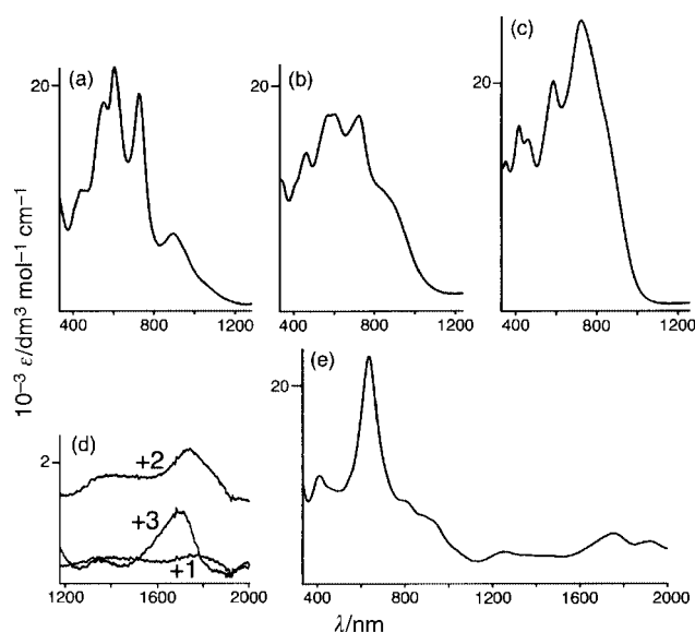
Fig. 8 Electronic spectra of [\text{Os}_2(\text{L}^2)]^{n+} ( n = 1, 2, 3 or 4 ) measured during a spectroelectrochemical experiment in MeCN at -30 \text{ }^\circ\text{C} . For clarity the spectra are shown individually. (a) n = 3 ; (b) n = 2 ; (c) n = 1 ; (d) near-IR region of n = 3, 2, 1 states overlaid; (e) n = 4 .
