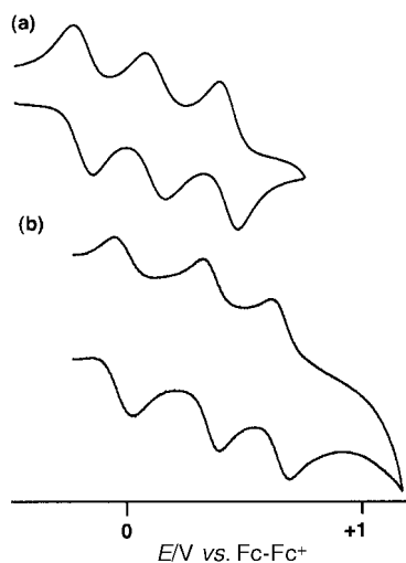
Fig. 5 Cyclic voltammograms of (a) [\text{Os}_3(\text{L}^3)]^{3+} and (b) [\text{Ru}_3(\text{L}^3)]^{3+} in MeCN (platinum working electrode; scan rate 0.2 \text{ V s}^{-1} ).
