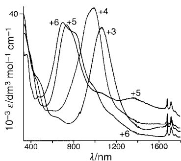
Fig. 9 Electronic spectra of [\text{Os}_n(\text{L}^3)]^{n+} ( n=3, 4, 5 or 6 ) measured during a spectroelectrochemical experiment in MeCN at -30\text{ }^\circ\text{C} .
