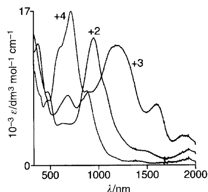
Fig. 7 Electronic spectra of [\text{Os}_2(\text{L}^1)]^{n+} ( n = 2, 3 or 4 ) measured during a spectroelectrochemical experiment in MeCN at -30 \text{ }^\circ\text{C} . Spectra of the n = 0 and 1 states could not be recorded due to deposition of the reduced forms of the complex on the electrode surface.
