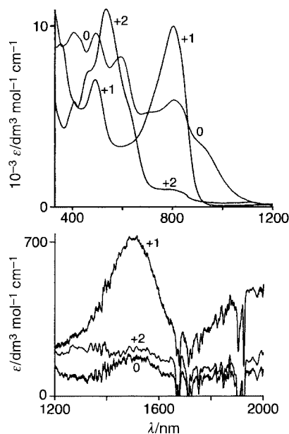
Fig. 2 Electronic spectra of [Os(bipy) 2 (cat)] n+ ( n = 0, 1 or 2 ) measured during a spectroelectrochemical experiment in MeCN at -30 °C.
